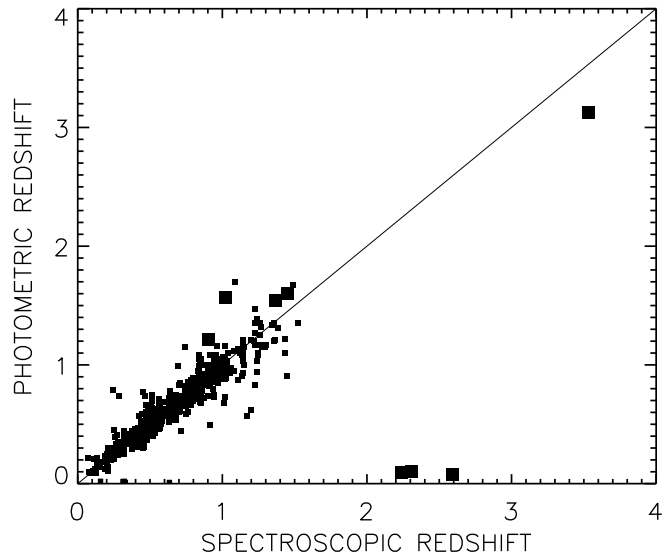
FIG. 14.— Photometric redshift versus spectroscopic redshift for the 1078 sources with R < 24 where both have been measured ( solid squares ). Objects with broad-line AGN spectra are distinguished with a larger symbol. Only 38 of the photometric redshifts differ by more than 30% from the spectroscopic redshift. Five of these cases are broad-line AGN.
